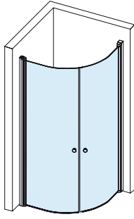
Kwart rond 2-delig 80 x 80 x 197 cm (781-791 mm) 90 x 90 x 197 cm (881-891 mm) 100 x 100 x 197 cm (981-991 mm)
