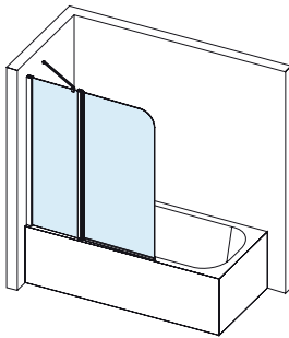
Badwand 2-delig 110 x 152 cm (1090-1100 mm) 130 x 152 cm (1290-1300 mm)
