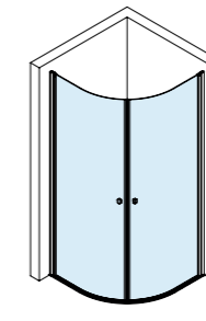
Kwartrond 90x90x200 cm (876-891x876-891 mm) 100x100x200 cm (976-991x976-991 mm)
